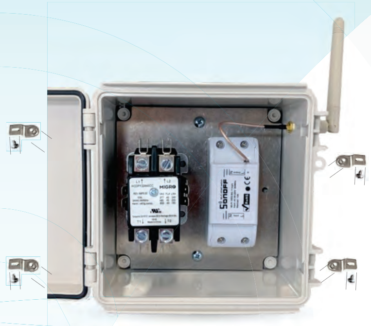
IMAGE 1. Mounting Brackets
